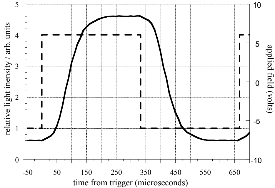
Figure 82: Ferroelectric electro-optic response.
