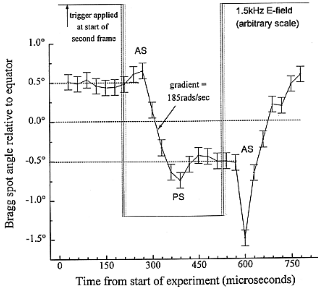
Figure 80: The angle of the Bragg diffraction spot relative to the equator, as a function of time during switching. Each data point represents the accumulated intensity in the preceding 30μs.
