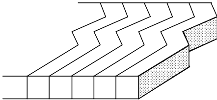
Figure 29: Emergence of a surface chevron structure due to E.F.T.
